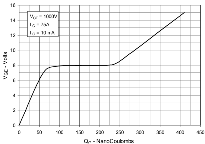
Fig. 7. Gate Charge
