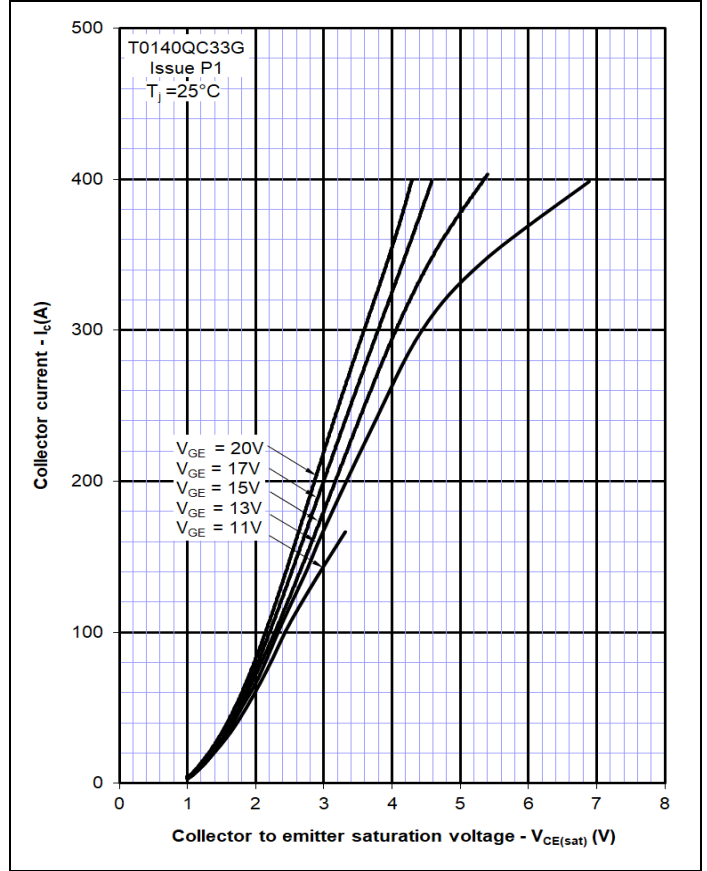
Figure 2 – Typical output characteristic
