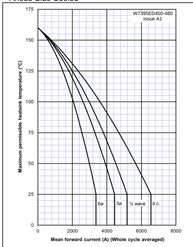
Figure 11 – Forward current vs. Heatsink temperature – Anode Side Cooled
