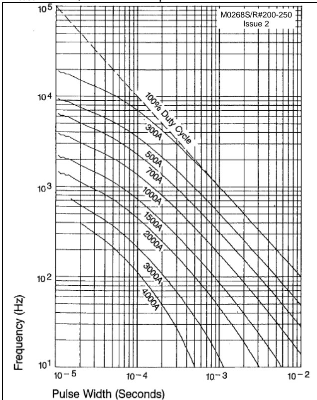
Figure 12 - Square wave frequency vs. pulse width, T_{case} - 60^{\circ}C , di/dt - 400A/\mu s
