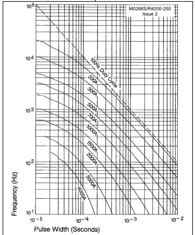
Figure 13 - Square wave frequency vs. pulse width, T_{case} - 90^{\circ}C , di/dt - 400A/\mu s
