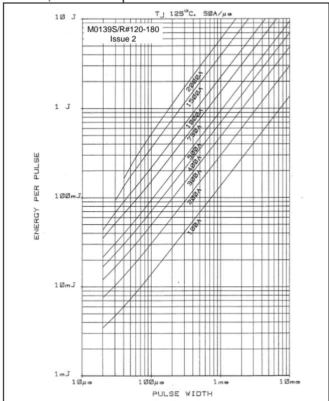
Figure 7 - Square wave energy per pulse, T J - 125°C, di/dt - 50A/µs
