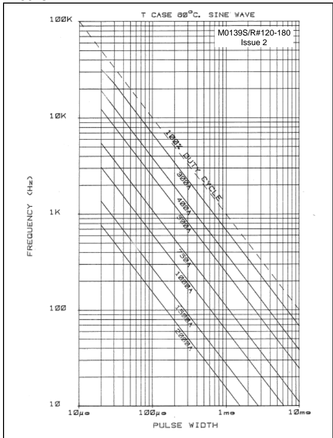
Figure 5 - Sine wave frequency vs. pulse width, T case - 60°C
