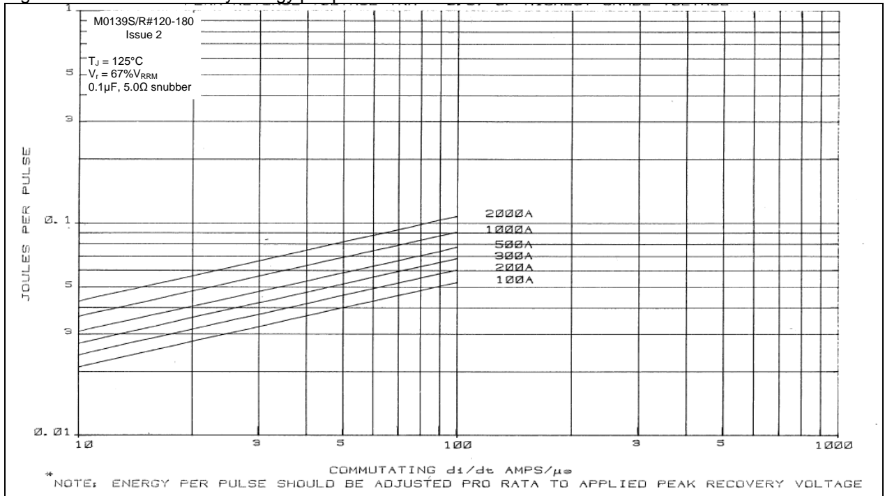
Figure 3 - Reverse recovery energy per pulse
