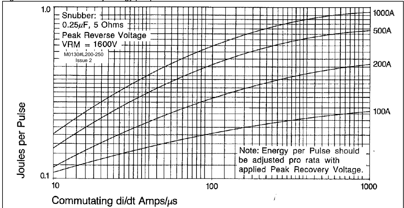
Figure 5 - Reverse recovery energy per pulse
