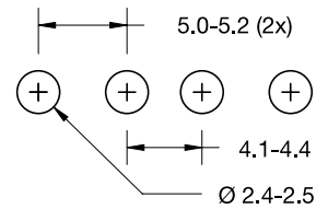
mounting pattern
