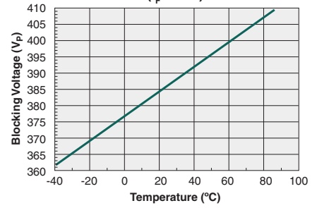
Form-B Typical Blocking Voltage vs. Temperature ( I_F=5mA )
