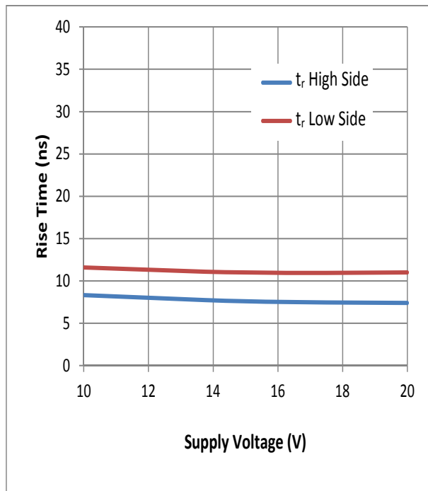
Figure 9. Rise Time vs. Supply Voltage
