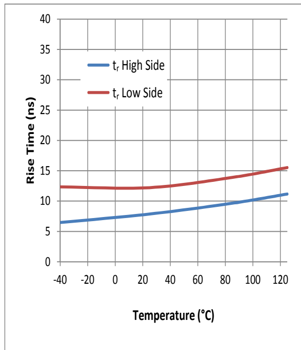
Figure 10. Rise Time vs. Temperature
