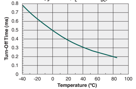
Form-A Typical Turn-Off Time vs. Temperature ( I_F=10mA, I_L=170mA_{DC} )
