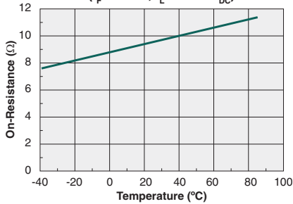
Form-A Typical On-Resistance vs. Temperature ( I_F=10mA, I_L=170mA_{DC} )
