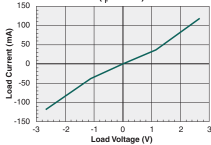
Form-A Typical Load Current vs. Load Voltage ( I_F=10mA )
