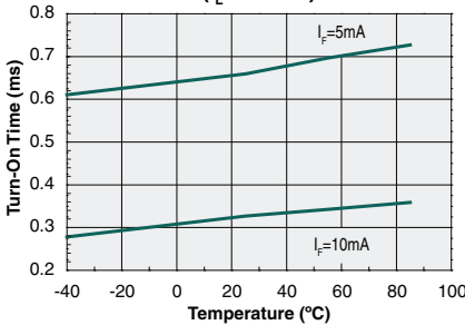
Turn-On Time vs. Temperature ( I_L=100mA )
