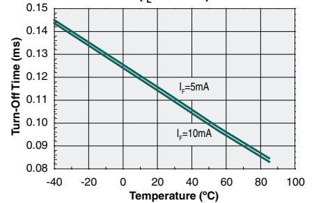
Turn-Off Time vs. Temperature ( I_L=100mA )
