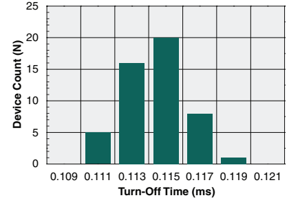
Typical Turn-Off Time Distribution (N=50, I_F=5mA , I_L=100mA )
