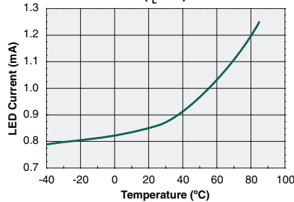
LED Current to Operate vs. Temperature ( I_L=1A )
