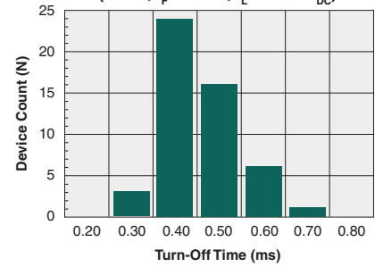
Typical Turn-Off Time (N=50, I_F=10\text{mA} , I_L=120\text{mA}_{DC} )
