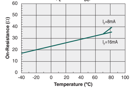
Typical On-Resistance vs. Temperature ( I_L=100mA_{DC} )
