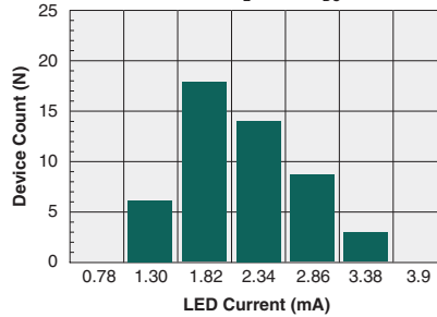
Typical I F for Switch Dropout (N=50, I L =85mA DC )
