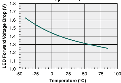
Typical LED Forward Voltage Drop vs. Temperature (I F =10mA)
