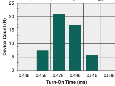
Typical Turn-On Time (N=50, I_F=2mA , I_L=120mA_{DC} )
