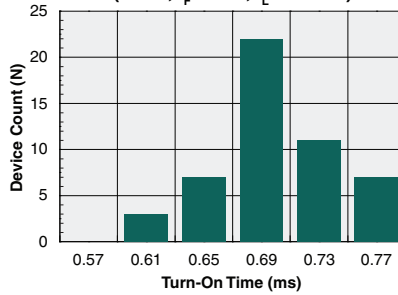
Form-A Typical Turn-On Time (N=50, I_F=5\text{mA} , I_L=100\text{mA} )
