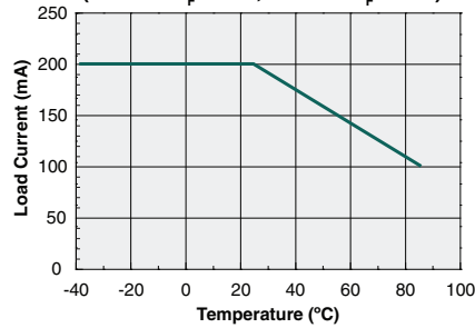
Load Current vs. Load Temperature (Form-A: I_F=5mA , Form-B: I_F=0mA )
