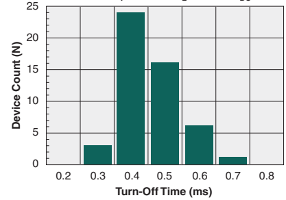
Typical Turn-Off Time (N=50, I_F=10mA , I_L=120mA_{DC} )
