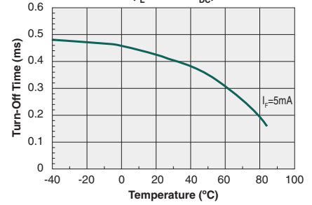
Typical Turn-Off Time vs. Temperature ( I_L=120mA_{DC} )
