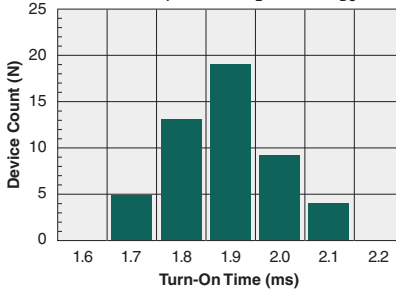
Typical Turn-On Time (N=50, I_F=10mA , I_L=120mA_{DC} )
