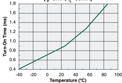
Typical Turn-On Time vs. Temperature ( I_F=5mA , I_L=80mA )
