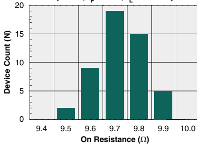
Typical On-Resistance Distribution (N=50, I_F=5mA , I_L=120mA )
