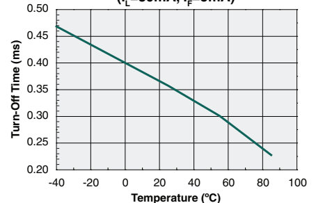
Typical Turn-Off Time vs. Temperature ( I_L=80mA , I_F=5mA )
