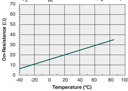
Typical On-Resistance vs. Temperature ( I_L=50mA_{DC} Instantaneous, I_F=5mA )
