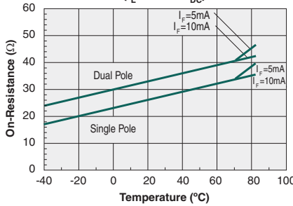
Typical On-Resistance vs. Temperature ( I_L=120mA_{DC} )
