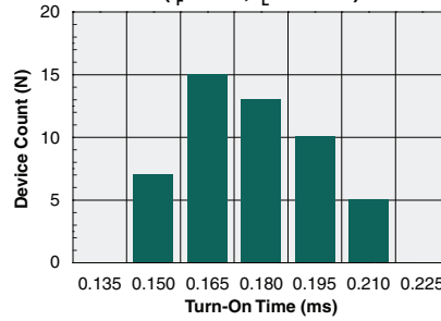
Turn-On Time Distribution ( I_F=5mA , I_L=200mA )
