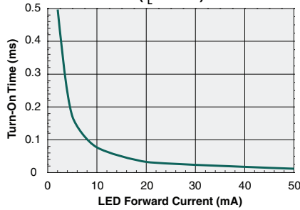
Turn-On Time vs. LED Forward Current ( I_L=80mA )
