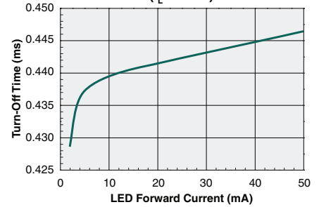
Turn-Off Time vs. LED Forward Current ( I_L=80mA )
