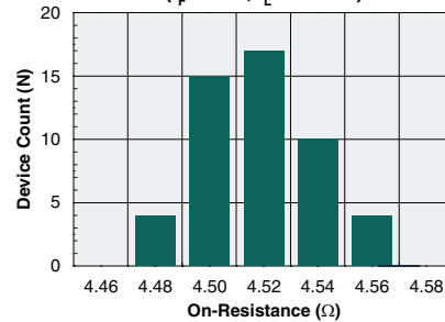
On-Resistance Distribution ( I_F=2mA , I_L=200mA )
