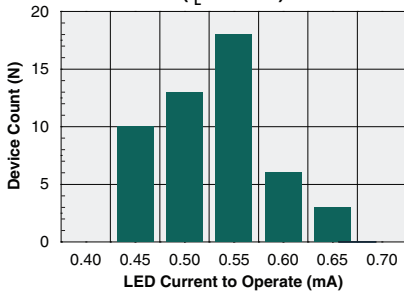
LED Current to Operate Distribution ( I_L=100mA )
