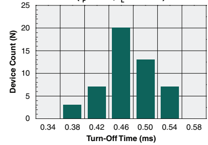
Turn-Off Time Distribution ( I_F=5mA , I_L=200mA )
