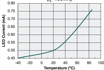
LED Current to Operate vs. Temperature ( I_L=100mA )
