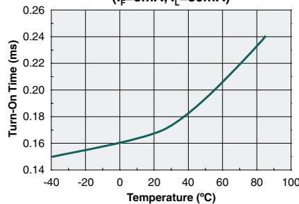
Turn-On Time vs. Temperature ( I_F=5mA , I_L=80mA )
