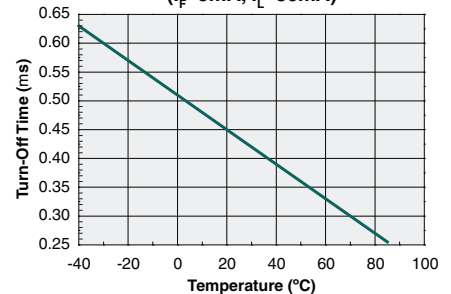
Turn-Off Time vs. Temperature ( I_F=5mA , I_L=80mA )
