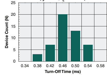
Turn-Off Time Distribution ( I_F=5mA , I_L=200mA )
