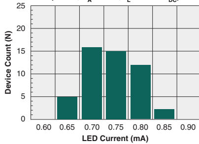
Typical I_F for Switch Operation (N=50, T_A=25^\circ C , I_L=120mA_{DC} )
