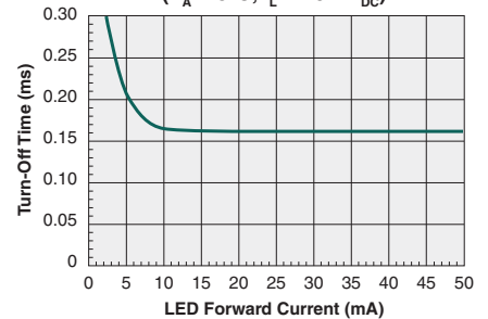
Typical Turn-Off Time vs. LED Forward Current ( T_A=25^\circ C , I_L=120mA_{DC} )
