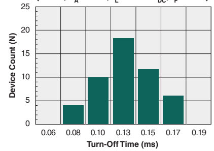
Typical Turn-Off Time (N=50, T_A=25^\circ C , I_L=120mA_{DC} , I_F=5mA )
