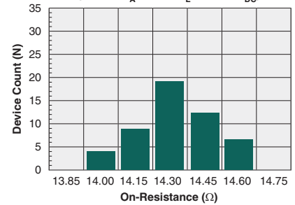
Typical On-Resistance Distribution (N=50, T_A=25^\circ C , I_L=120mA_{DC} )
