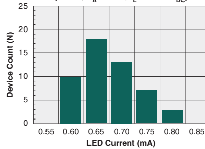
Typical I_F for Switch Dropout (N=50, T_A=25^\circ C , I_L=120mA_{DC} )
