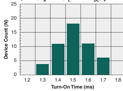
Typical Turn-On Time (N=50, T_A=25^\circ C , I_L=120mA_{DC} , I_F=5mA )
