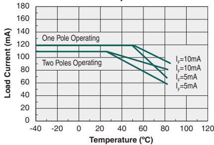
Maximum Continuous DC Load Current vs. Temperature
