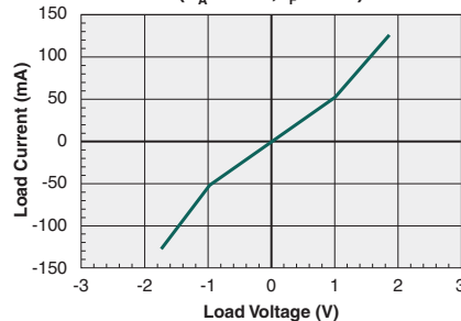
Typical Load Current vs. Load Voltage ( T_A=25°C , I_F=5mA )
