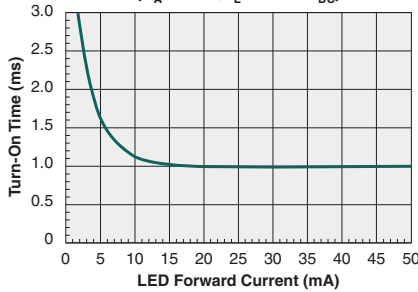
Typical Turn-On Time vs. LED Forward Current ( T_A=25^\circ\text{C} , I_L=120\text{mA}_{DC} )
