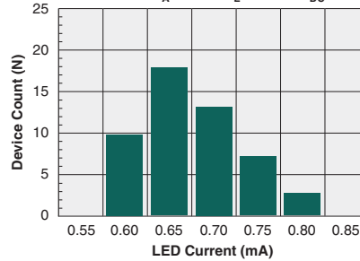
Typical I_F for Switch Dropout (N=50, T_A=25^\circ\text{C} , I_L=120\text{mA}_{DC} )
