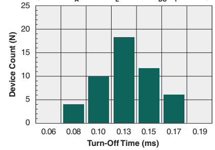
Typical Turn-Off Time (N=50, T_A=25^\circ\text{C} , I_L=120\text{mA}_{DC} , I_F=5\text{mA} )
