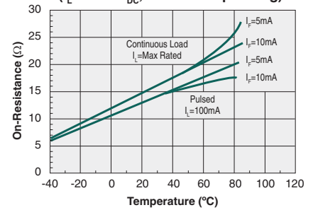
Typical On-Resistance vs. Temperature ( I_L=120mA_{DC} , One Pole Operating)
