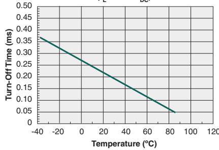
Typical Turn-Off Time vs. Temperature ( I_L=70mA_{DC} )
