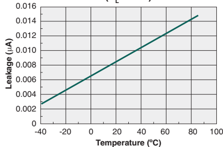
Typical Leakage vs. Temperature Measured across Pins 5&6, 7&8 ( V_L=350V )
