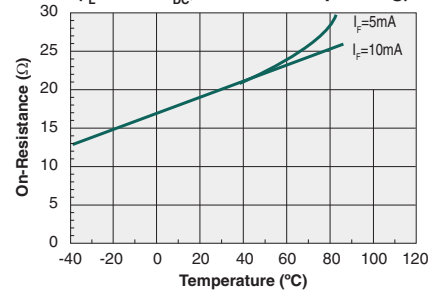
Typical On-Resistance vs. Temperature ( I_L=120mA_{DC} , Both Poles Operating)
