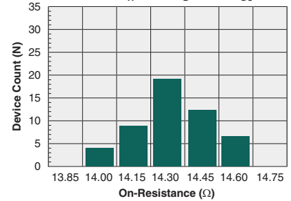
Typical On-Resistance Distribution (N=50, T_A=25^\circ\text{C} , I_L=120\text{mA}_{DC} )
