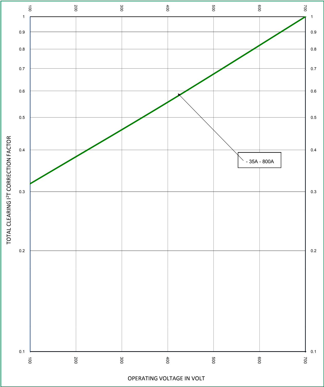
Total Clearing I²t Correction Factor Curve L70QS Series
