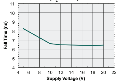
Fall Time vs. Supply Voltage ( C_L=1.8nF )
