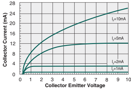
Typical Transfer Characteristics of Single Transistor Detector
