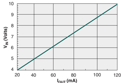
V-I Characteristics for Test Circuit
