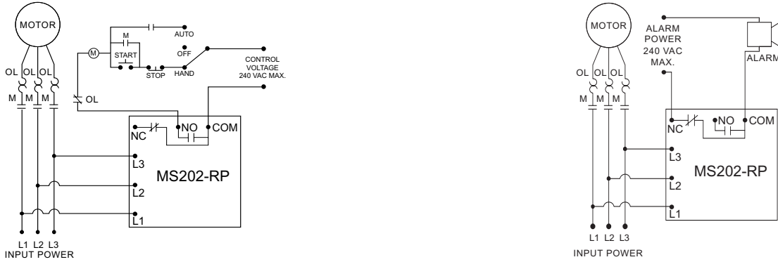
Figure No. 1: Typical Wiring Diagram
