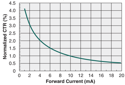
Typical Normalized CTR vs. Forward Current ( V_{CE}=0.5V )
