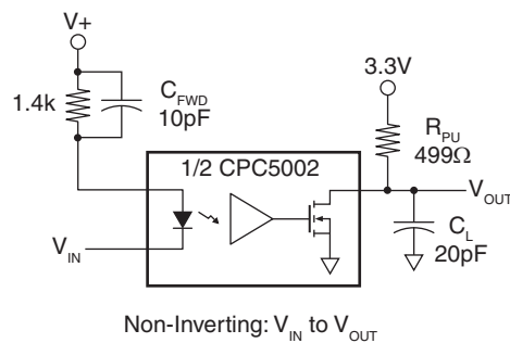
Figure 2. Non-Inverting Configuration
