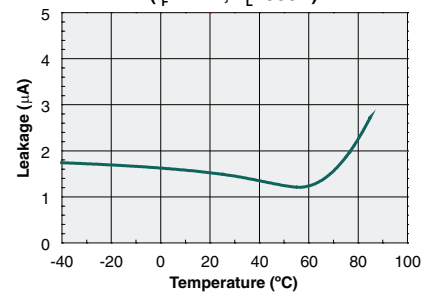
Leakage Current vs. Temperature Measured Across Pins 7 & 8 ( I_F=2mA, V_L=350V )
