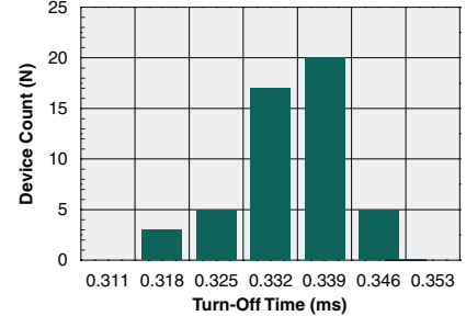
Typical Turn-Off Time (N=50, I_F=5mA , I_L=60mA )
