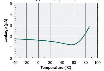
Leakage Current vs. Temperature Measured Across Pins 7 & 8 ( I_F=2\text{mA} , V_L=350\text{V} )
