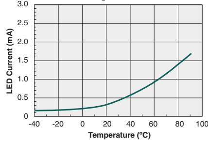
Typical I_F for Switch Operation vs. Ambient Temperature ( I_L=80\text{mA} )
