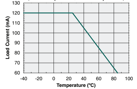
Maximum Load Current vs. Ambient Temperature (Form-A I_F=2\text{mA} , Form-B I_F=0\text{mA} )
