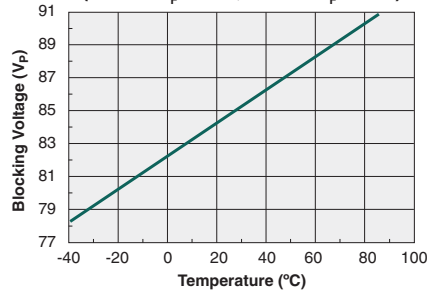
Typical Blocking Voltage vs. Ambient Temperature (Form-A I_F=0\text{mA} , Form-B I_F=2\text{mA} )
