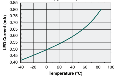
Typical I_F for Switch Operation ( I_L=60mA )
