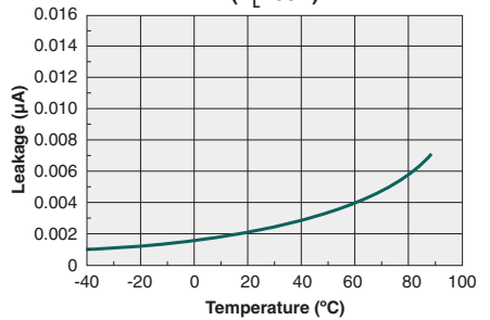
Typical Leakage vs. Temperature Measured Across Pins 5&6 and 7&8 ( V_L=60V )
