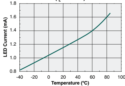
Typical I_F for Switch Operation ( I_L=300\text{mA} )
