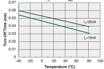
Typical Turn-Off Time vs. Temperature (I L =100mA DC )
