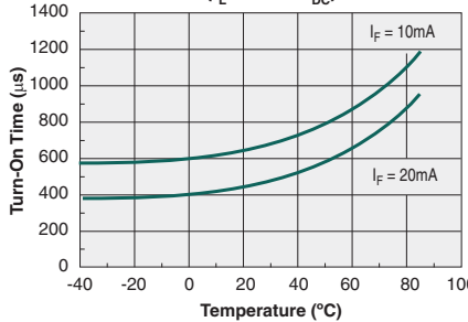
Typical Turn-On Time vs. Temperature (I L =100mA DC )
