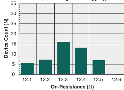
Typical On-Resistance Distribution (N=50, I F =5mA, I L =120mA DC , T A =25°C)
