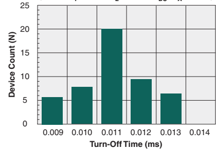
Typical Turn-Off Time (N=50, I F =5mA, I L =120mA DC , T A =25°C)
