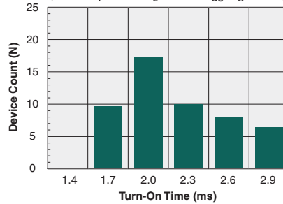
Typical Turn-On Time (N=50, I F =5mA, I L =120mA DC , T A =25°C)
