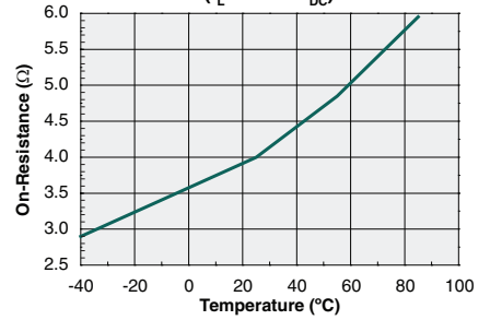
Typical On-Resistance vs. Temperature ( I_L = 100\text{mA}_{DC} )
