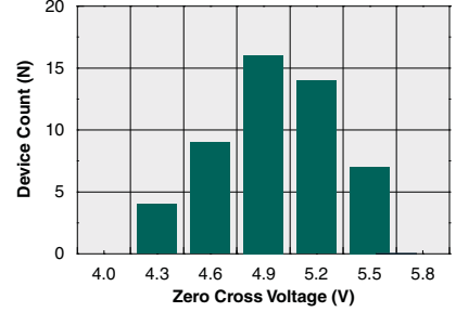
Zero Cross Voltage Distribution (N=50, I F =5mA)
