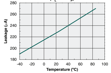
Typical Leakage vs. Temperature (V L =600V p )
