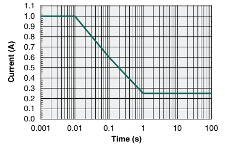
Maximum Non-Repetitive Surge Current ( T_A=25^\circ\text{C} )
