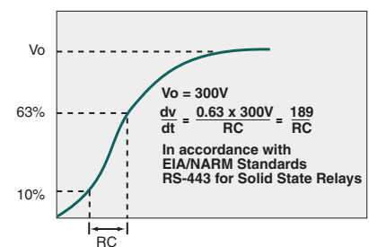
dV/dt Method
