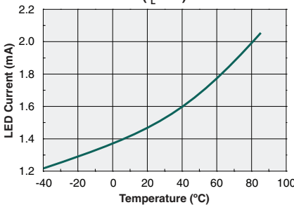
Typical I_F for Switch Operation ( I_L=1A )
