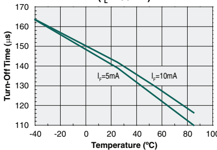
Typical Turn-Off Time vs. Temperature ( I_L=100mA )
