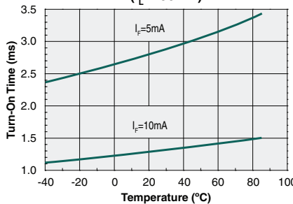
Typical Turn-On Time vs. Temperature ( I_L=100mA )
