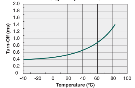
Typical Turn-Off vs. Temperature ( V_{IN}=5V , I_L=100mA )
