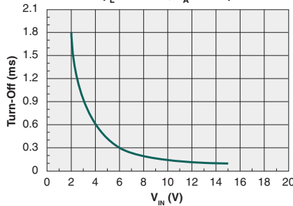
Typical Turn-Off vs. V_{IN} ( I_L=100mA , T_A=25^\circ C )
