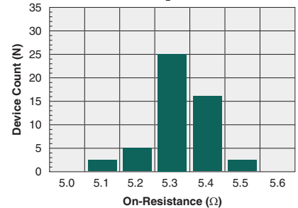
Typical On-Resistance Distribution (N=50, I_L=150mA )
