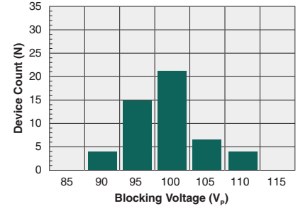
Typical Blocking Voltage Distribution (N=50, I_F=1mA )
