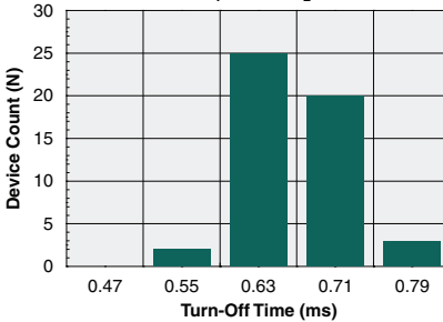
Typical Turn-Off Time Distribution (N=50, I F =5mA, I L =5mA)
