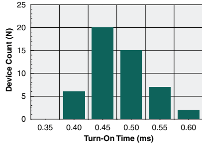
Typical Turn-On Time Distribution (N=50, I F =5mA, I L =5mA)
