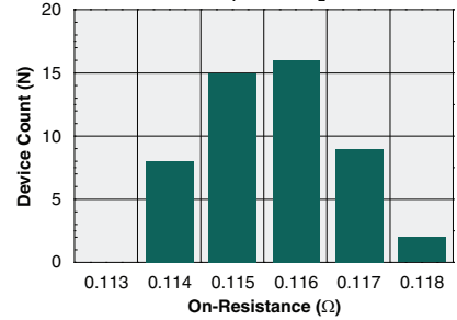
Typical On-Resistance Distribution (N=50, I F =2mA, I L =1A)
