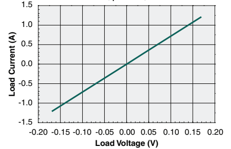
Typical Load Voltage vs. Load Current (I F =2mA)
