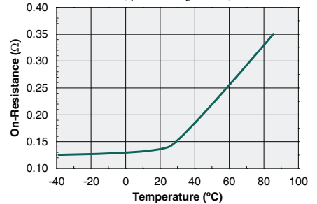
Typical On-Resistance vs. Temperature (I F =2mA, I L =0.5A)
