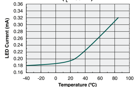
Typical I_F for Switch Dropout vs. Temperature ( I_L=480\text{mA} )
