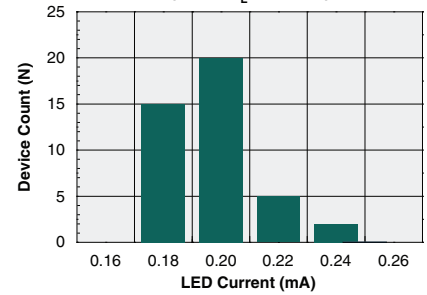
Typical I_F for Switch Dropout (N=50, I_L=600\text{mA} )
