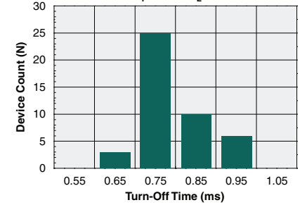
Typical Turn-Off Time (N=50, I_F=5mA , I_L=100mA )
