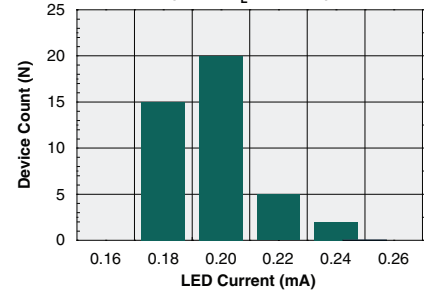
Typical I_F for Switch Dropout (N=50, I_L=400mA )
