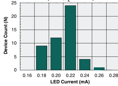
Typical I_F for Switch Operation (N=50, I_L=400mA )
