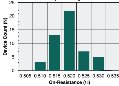
Typical On-Resistance Distribution (N=50, I_F=1mA , I_L=400mA )
